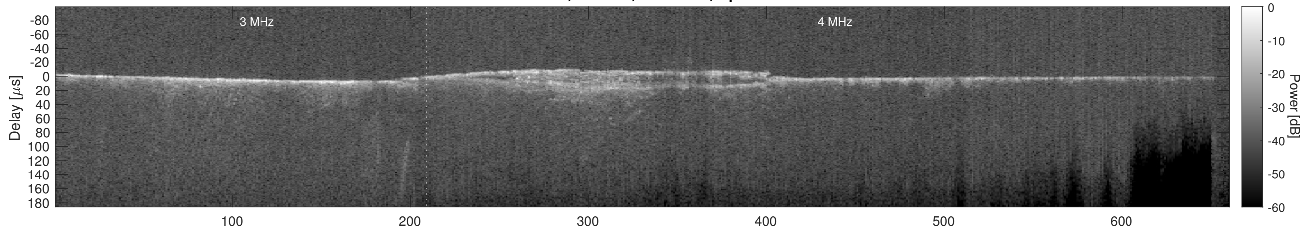
Orbit 7557, Cluttergram
