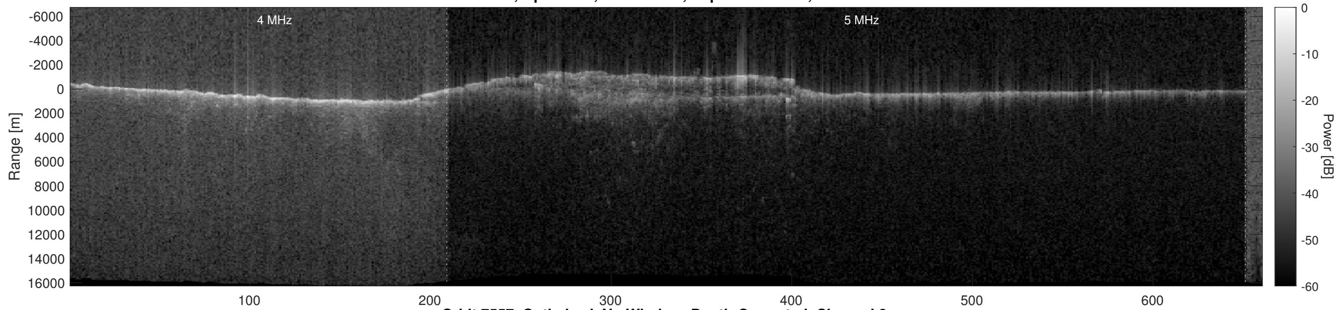
Orbit 7557, Optimized, No Window, Depth-Corrected, Channel 2
