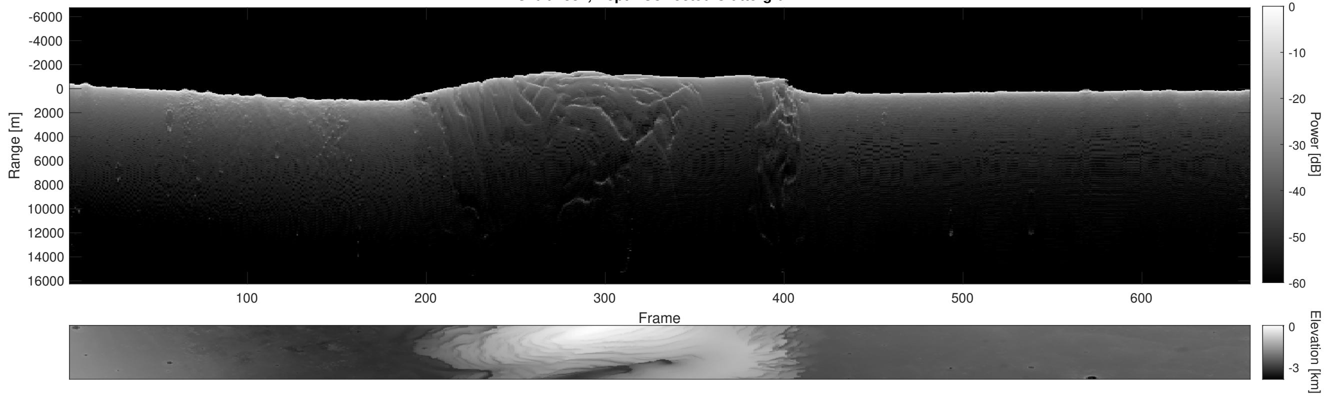
Orbit 7557, Depth-Corrected Cluttergram
