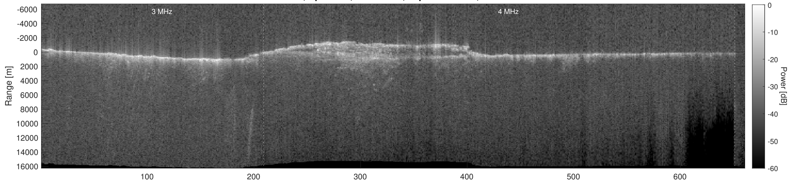
Orbit 7557, Depth-Corrected Cluttergram
