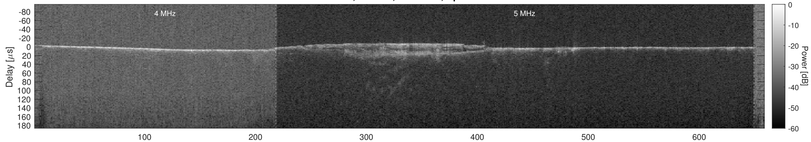
Orbit 7564, Cluttergram
