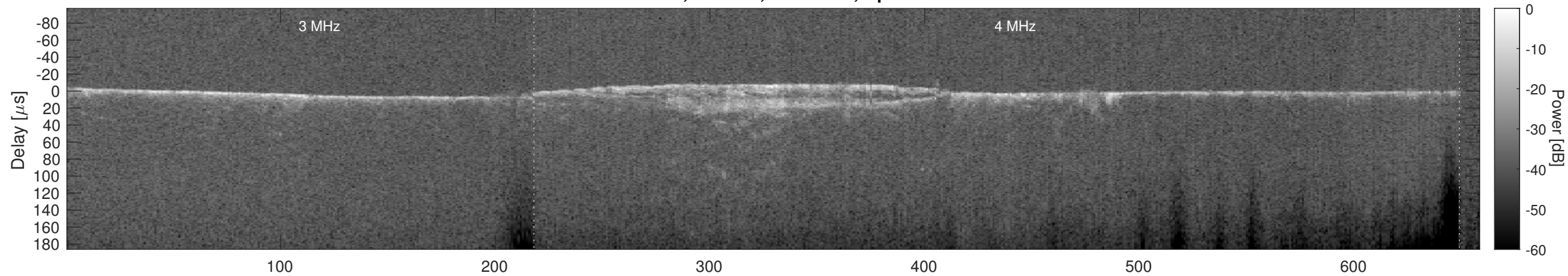
Orbit 7564, Cluttergram
