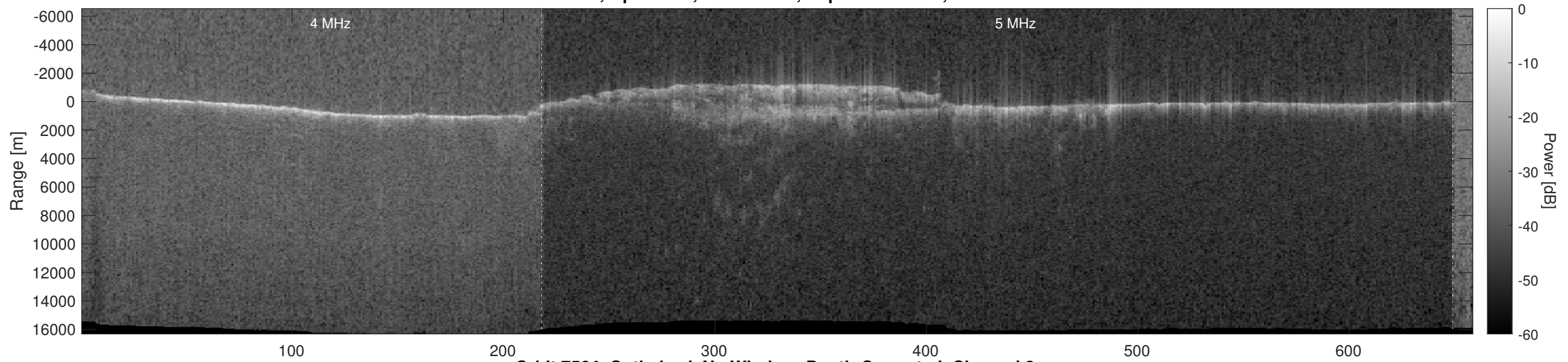
Orbit 7564, Optimized, No Window, Depth-Corrected, Channel 2
