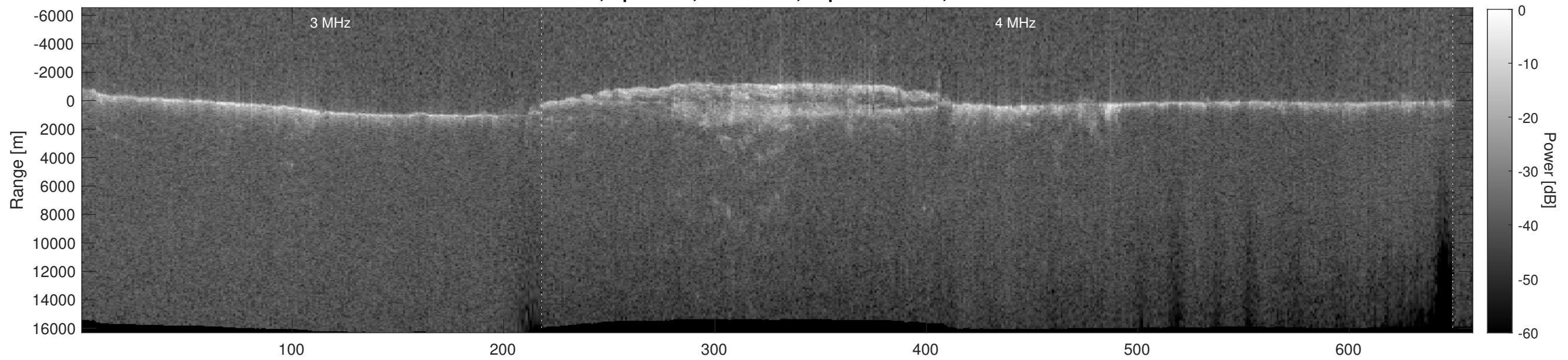
Orbit 7564, Depth-Corrected Cluttergram
