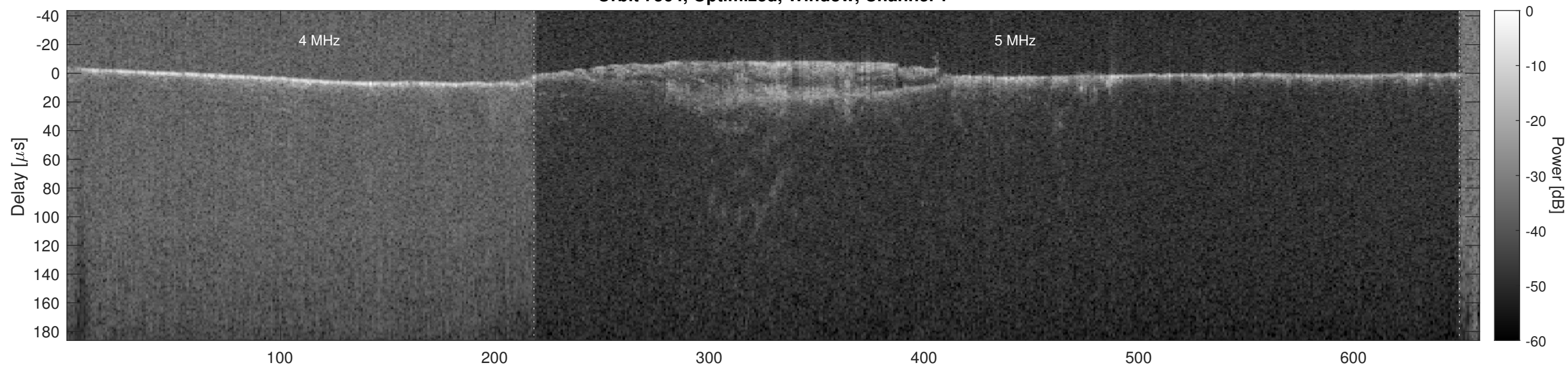
Orbit 7564, Optimized, Window, Channel 2
