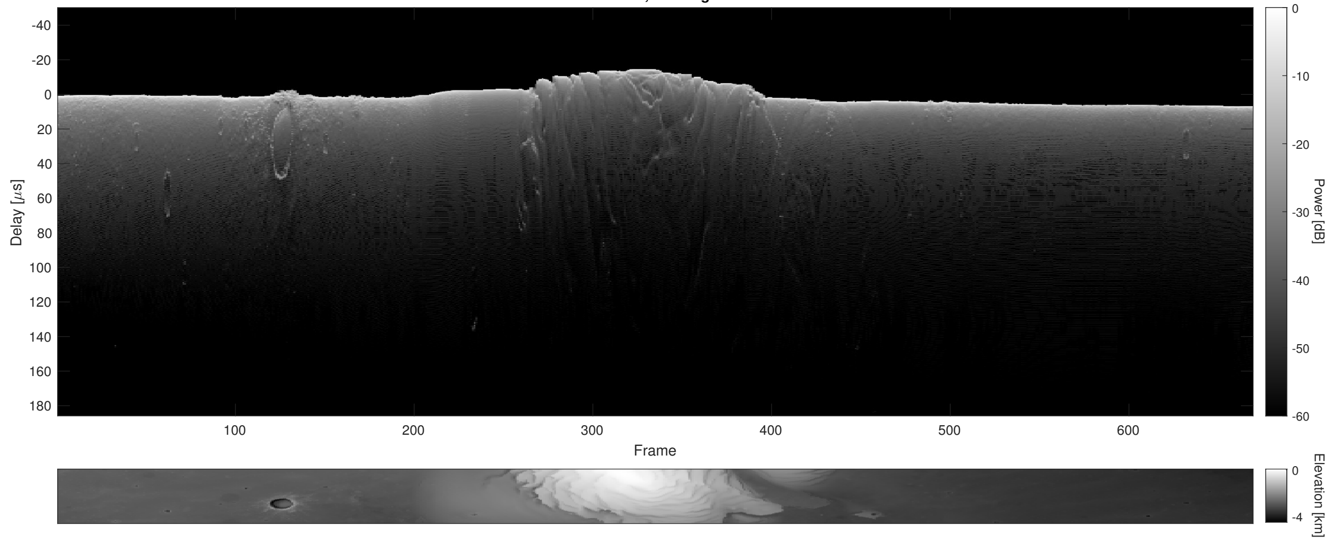
Orbit 7565, Cluttergram
