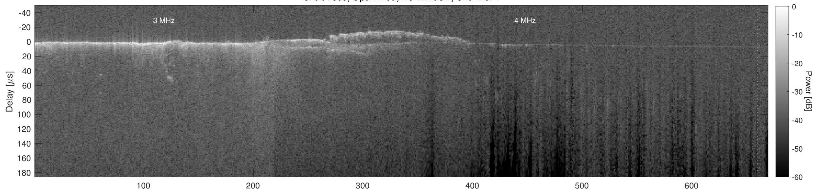
Orbit 7565, Cluttergram
