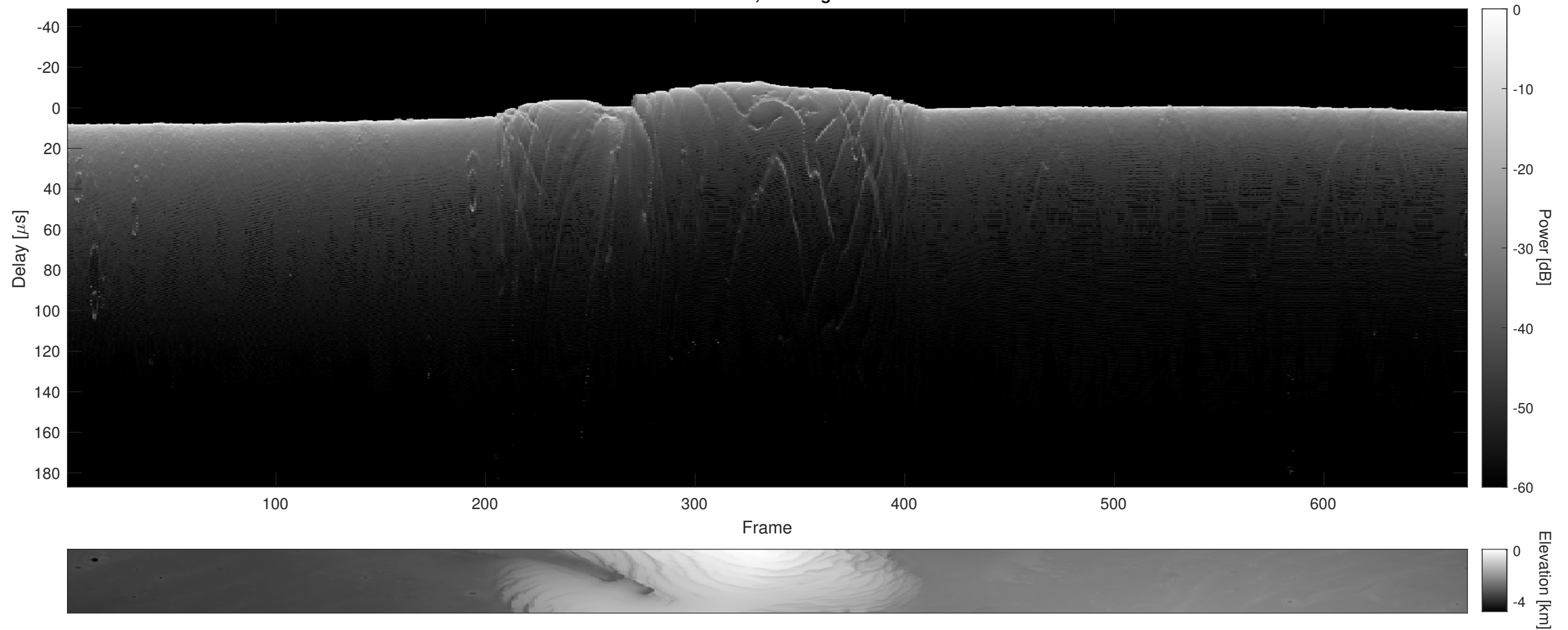
Orbit 7567, Cluttergram
