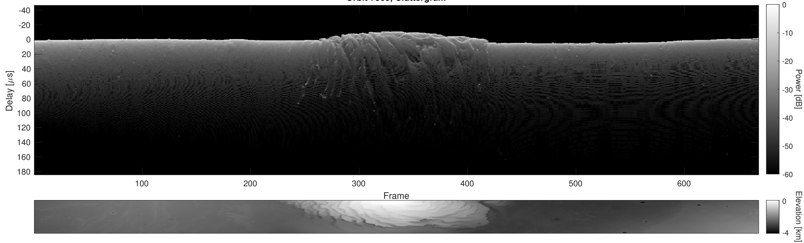
Orbit 7569, Cluttergram
