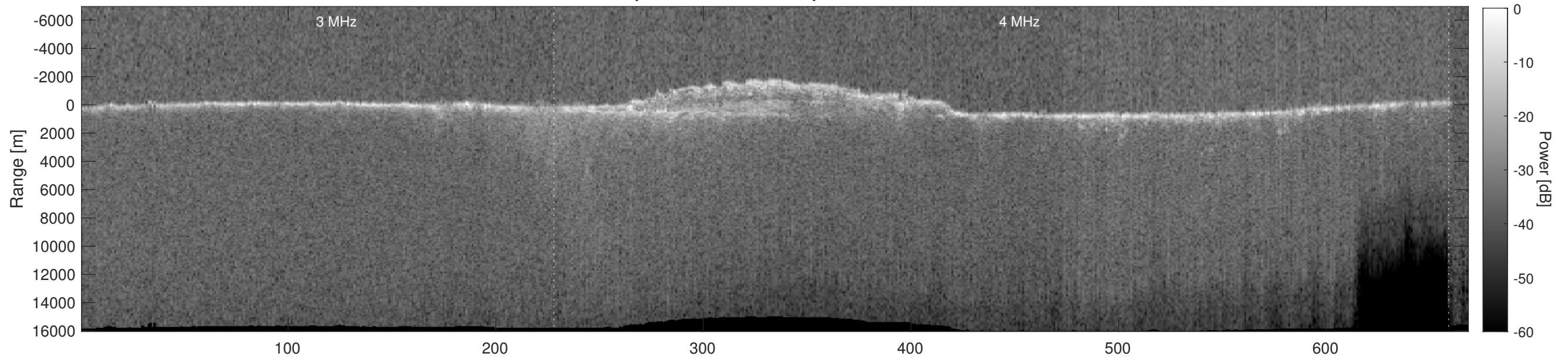
Orbit 7569, Depth-Corrected Cluttergram
