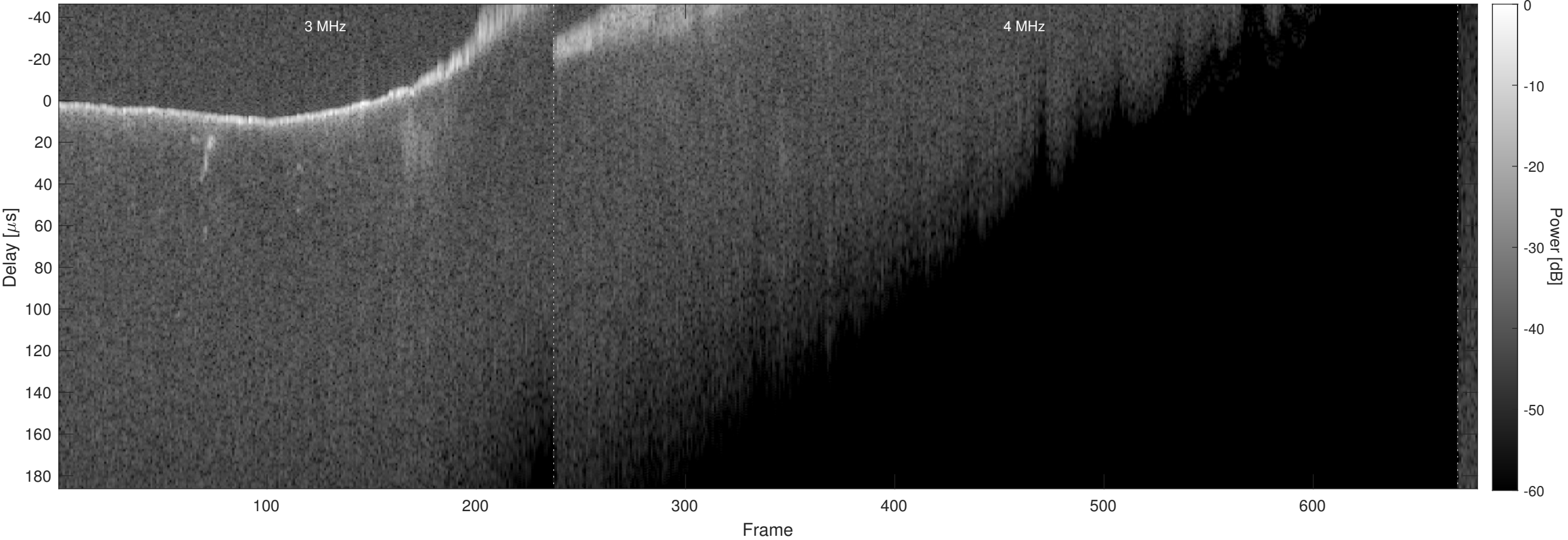
Orbit 7578, Chapman, Window, Channel 2
