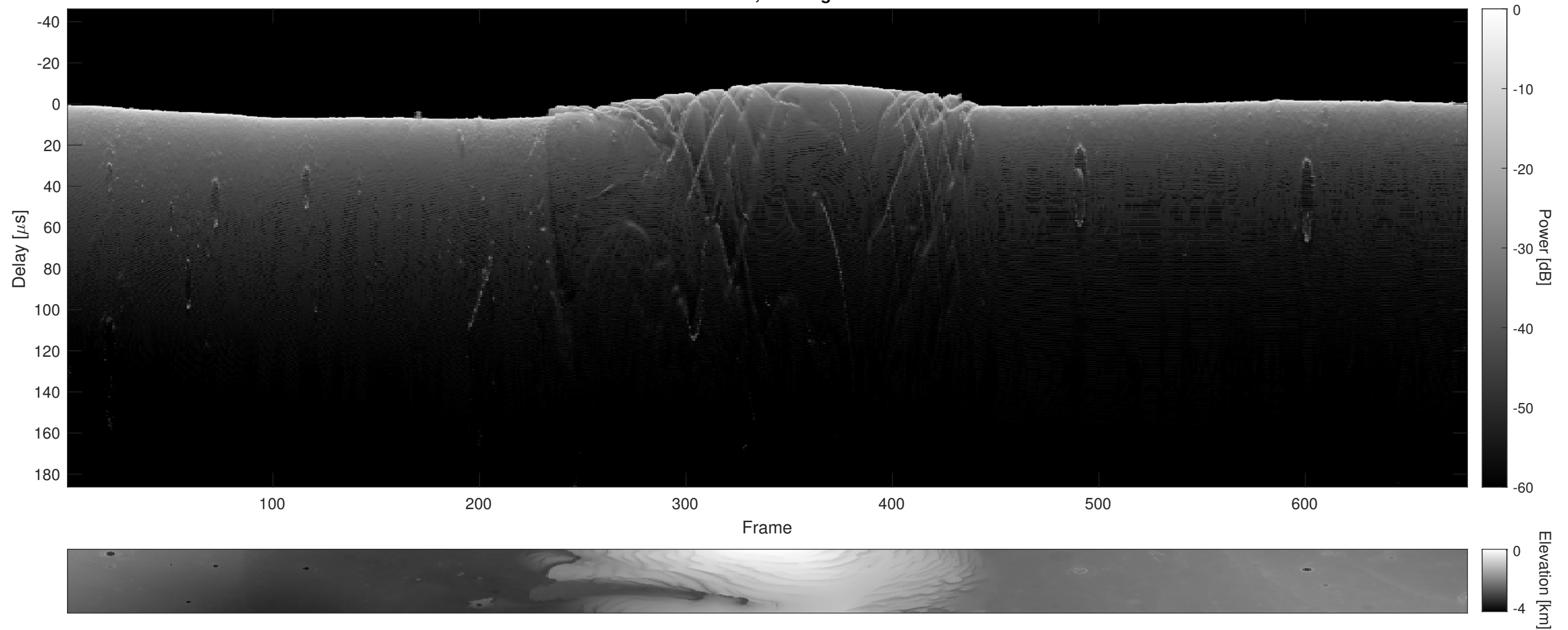
Orbit 7578, Cluttergram
