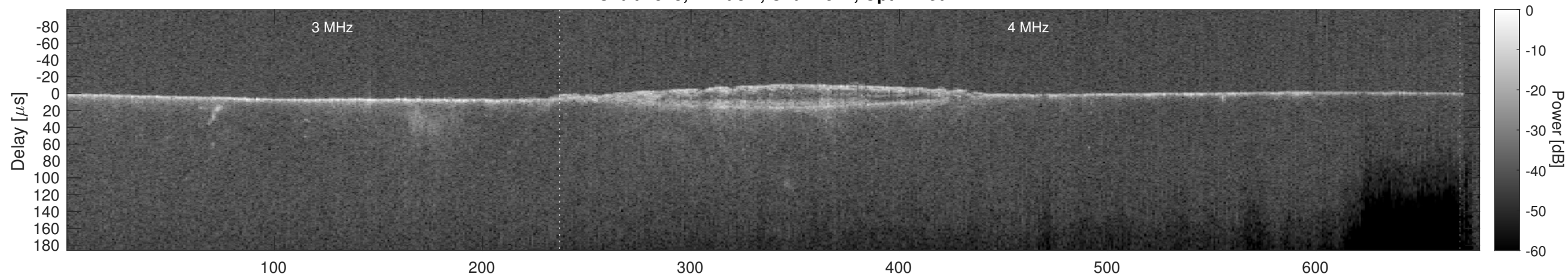
Orbit 7578, Cluttergram
