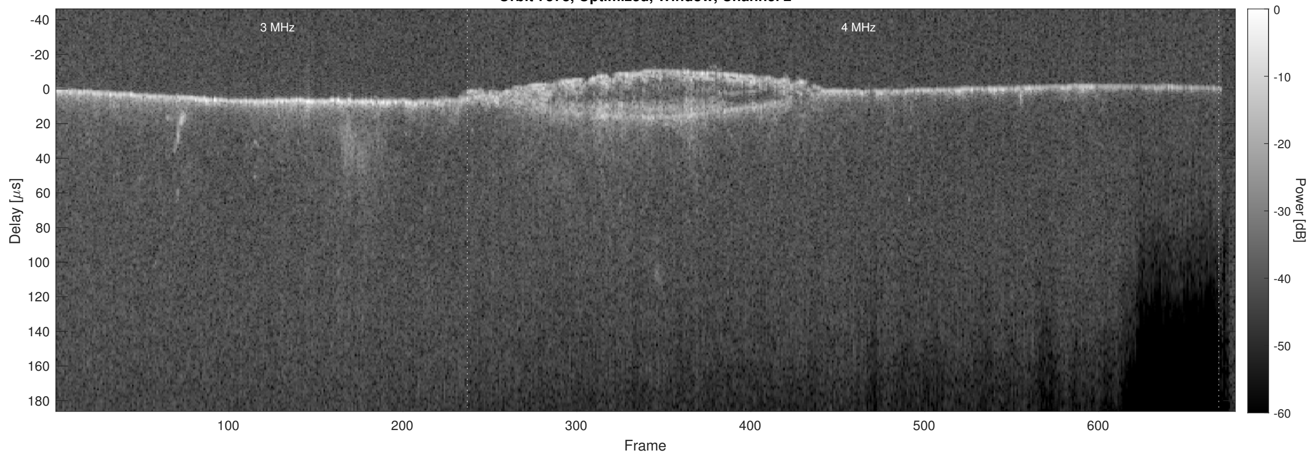
Orbit 7578, Optimized, Window, Channel 2
