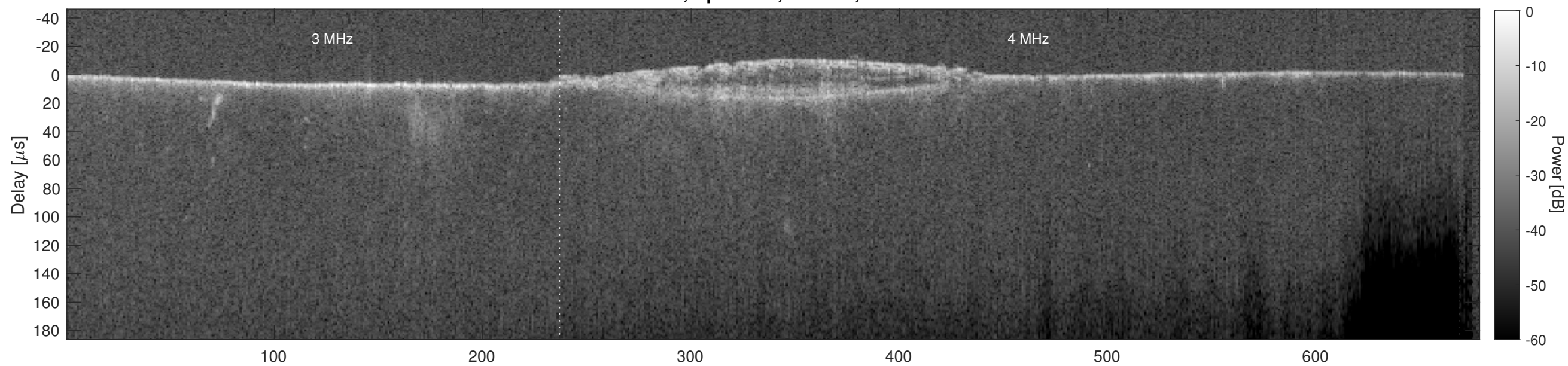
Orbit 7578, Cluttergram
