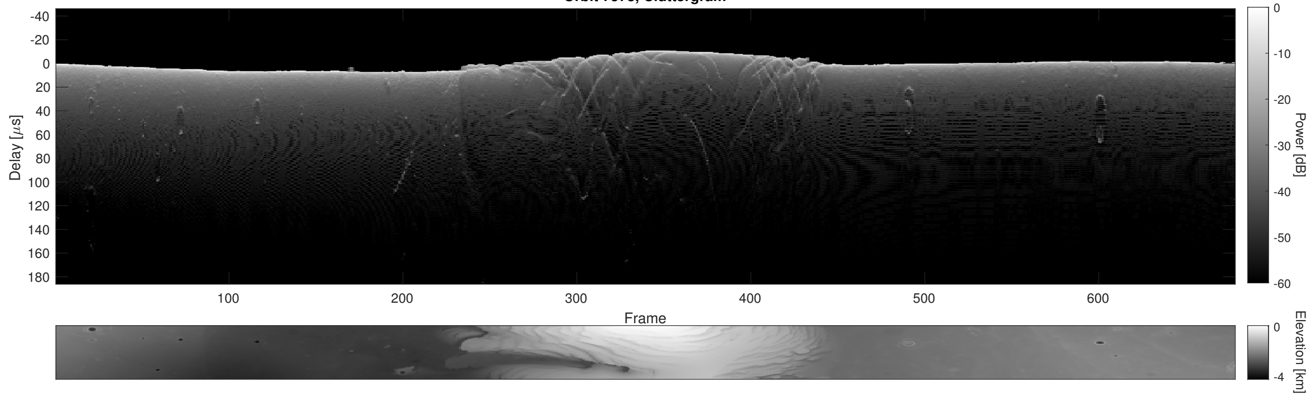
Orbit 7578, Cluttergram
