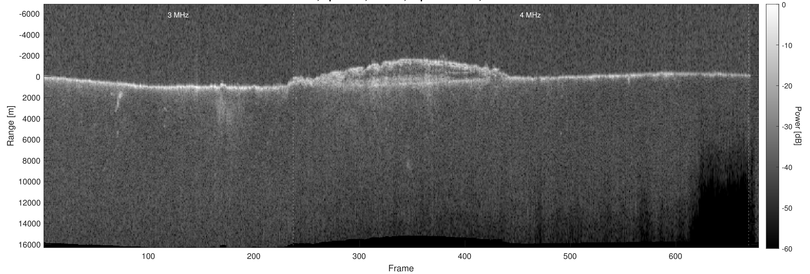
Orbit 7578, Optimized, Window, Depth-Corrected, Channel 2
