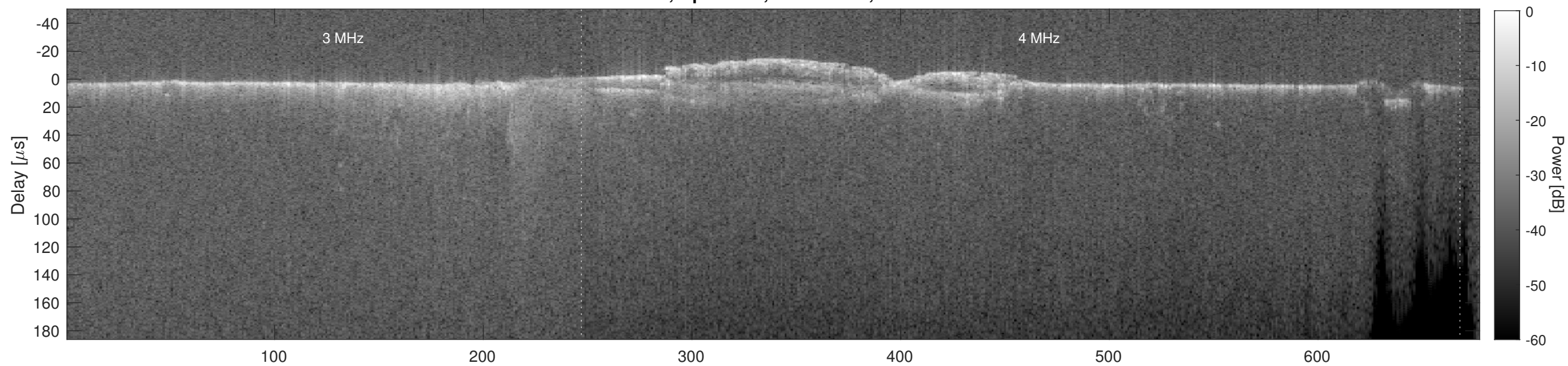
Orbit 7579, Cluttergram
