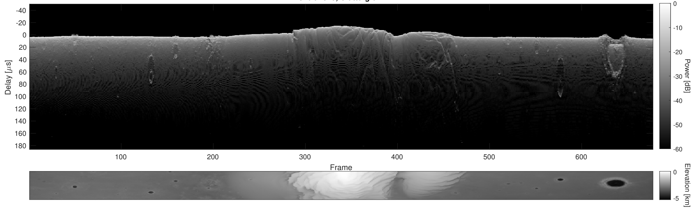
Orbit 7579, Cluttergram
