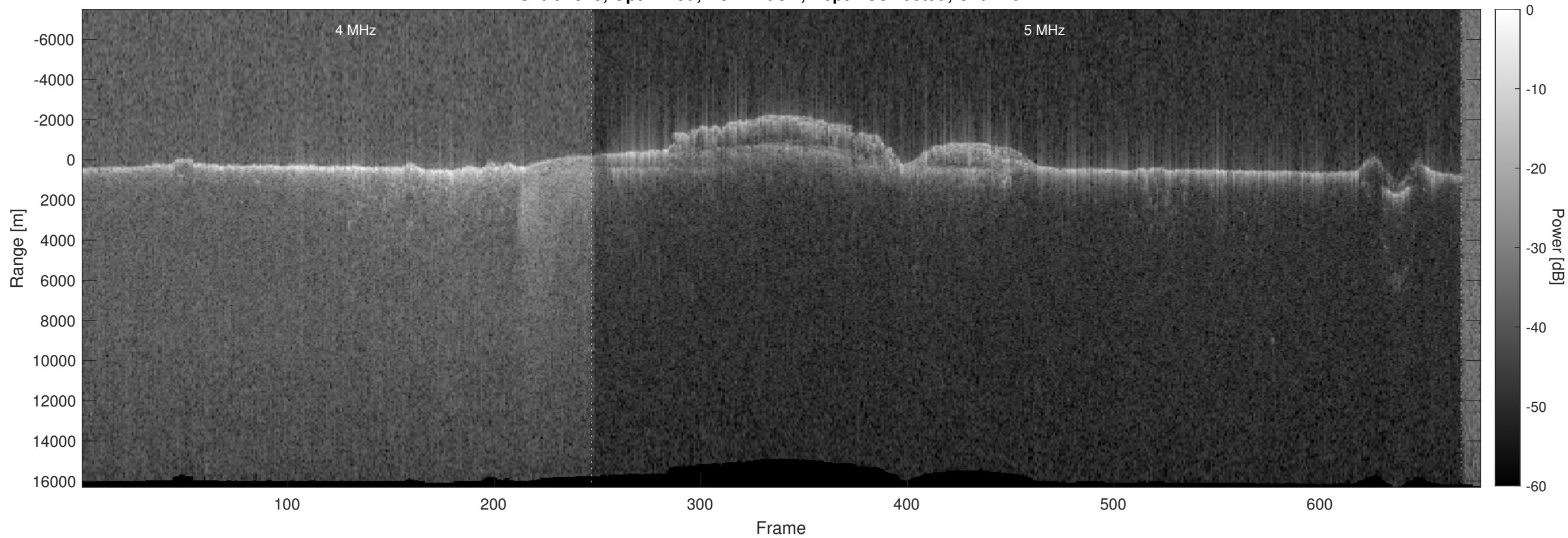
Orbit 7579, Optimized, No Window, Depth-Corrected, Channel 2
