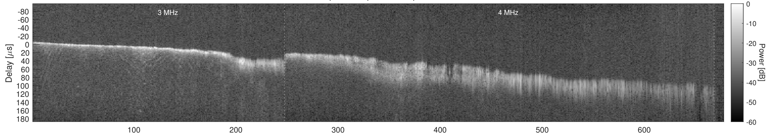
Orbit 7582, Window, Channel 2, Chapman
