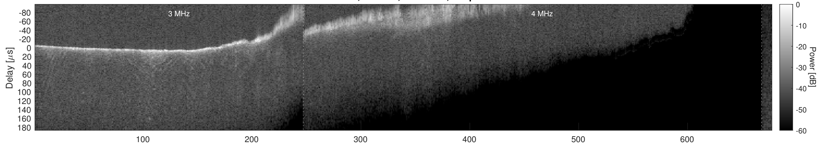
Orbit 7582, Window, Channel 2, Optimized
