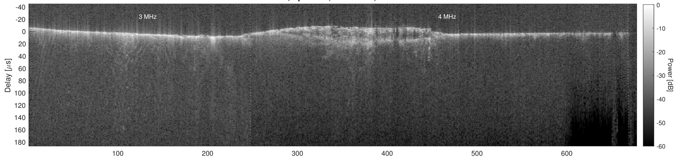
Orbit 7582, Cluttergram
