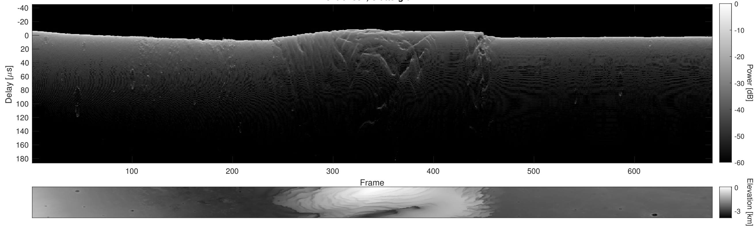
Orbit 7582, Cluttergram
