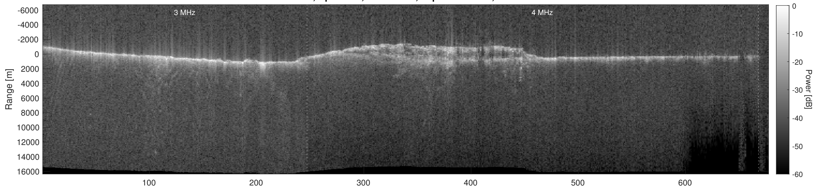
Orbit 7582, Depth-Corrected Cluttergram
