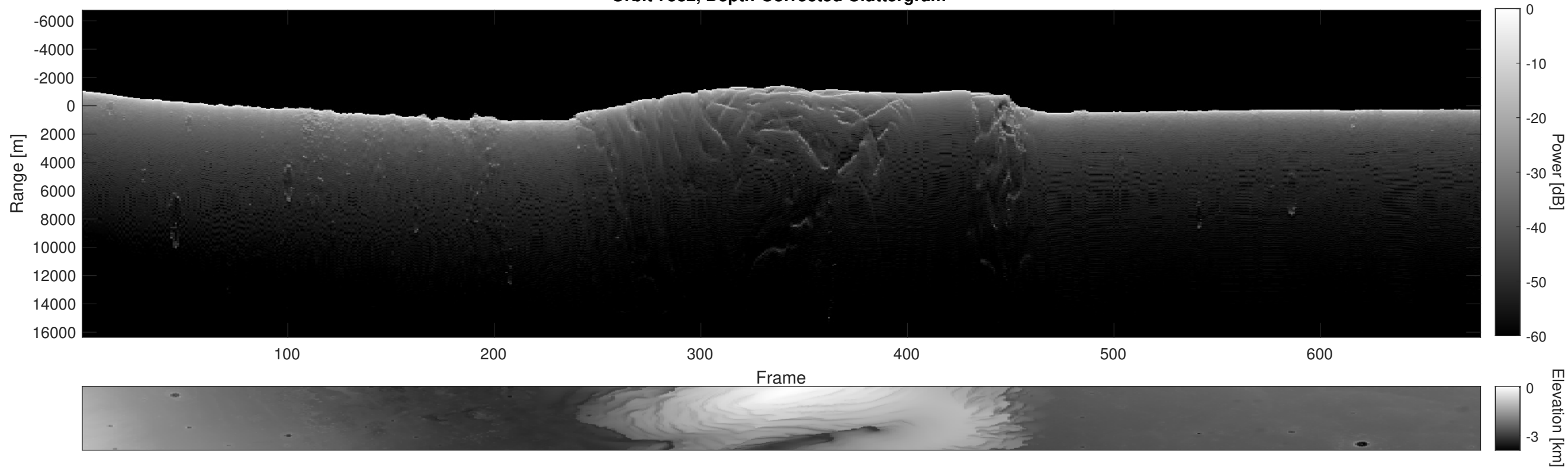
Orbit 7582, Depth-Corrected Cluttergram
