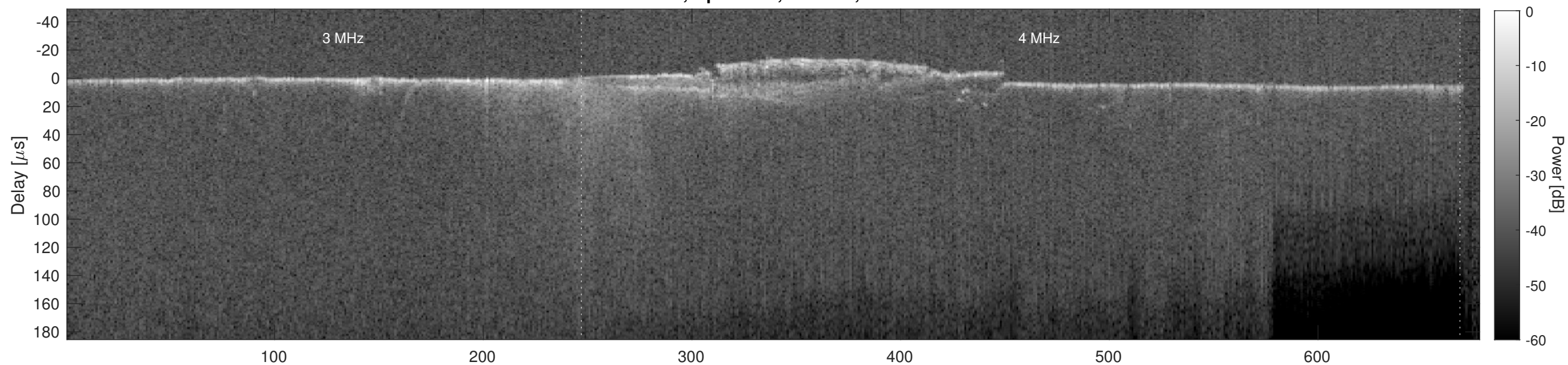
Orbit 7583, Cluttergram
