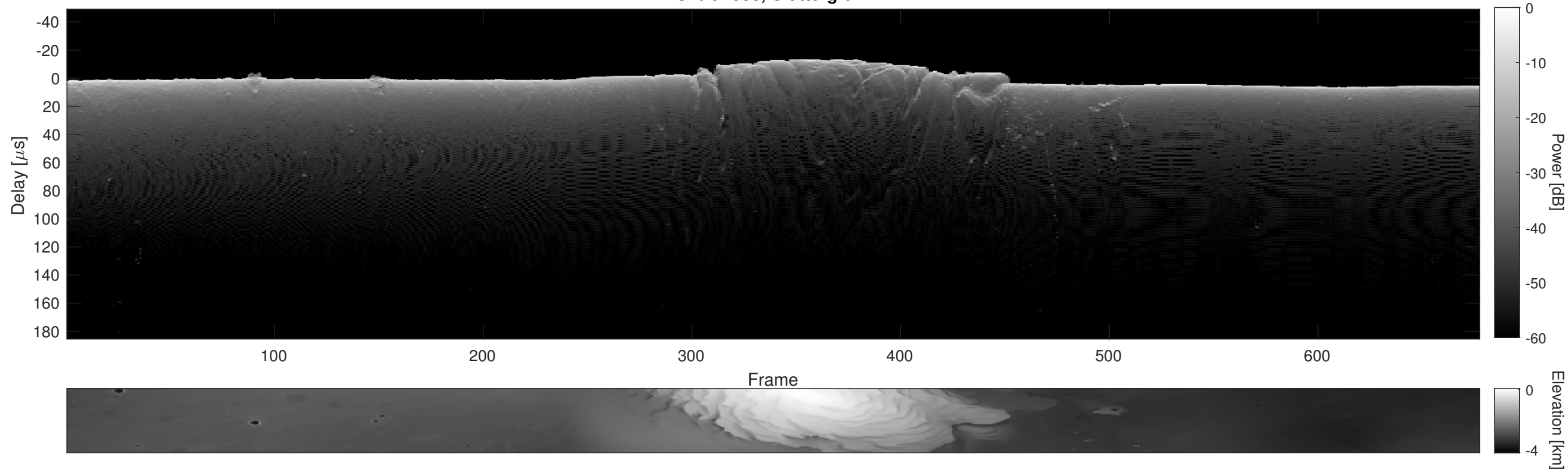
Orbit 7583, Cluttergram
