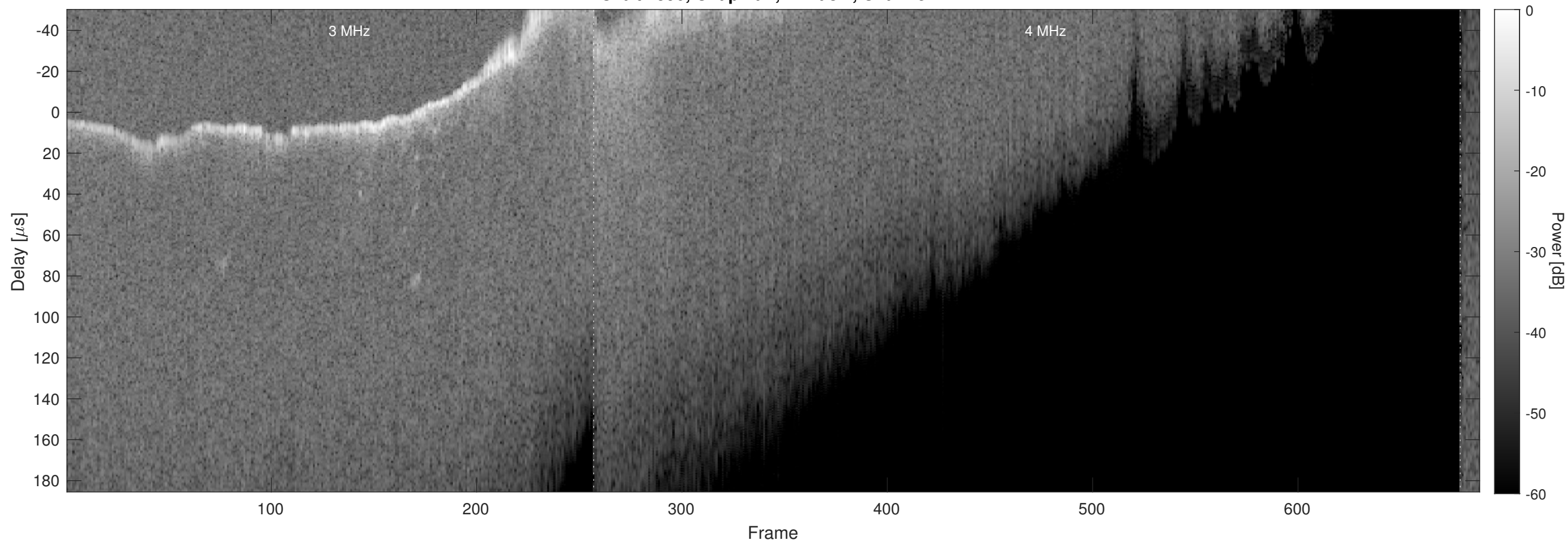
Orbit 7590, Chapman, Window, Channel 2
