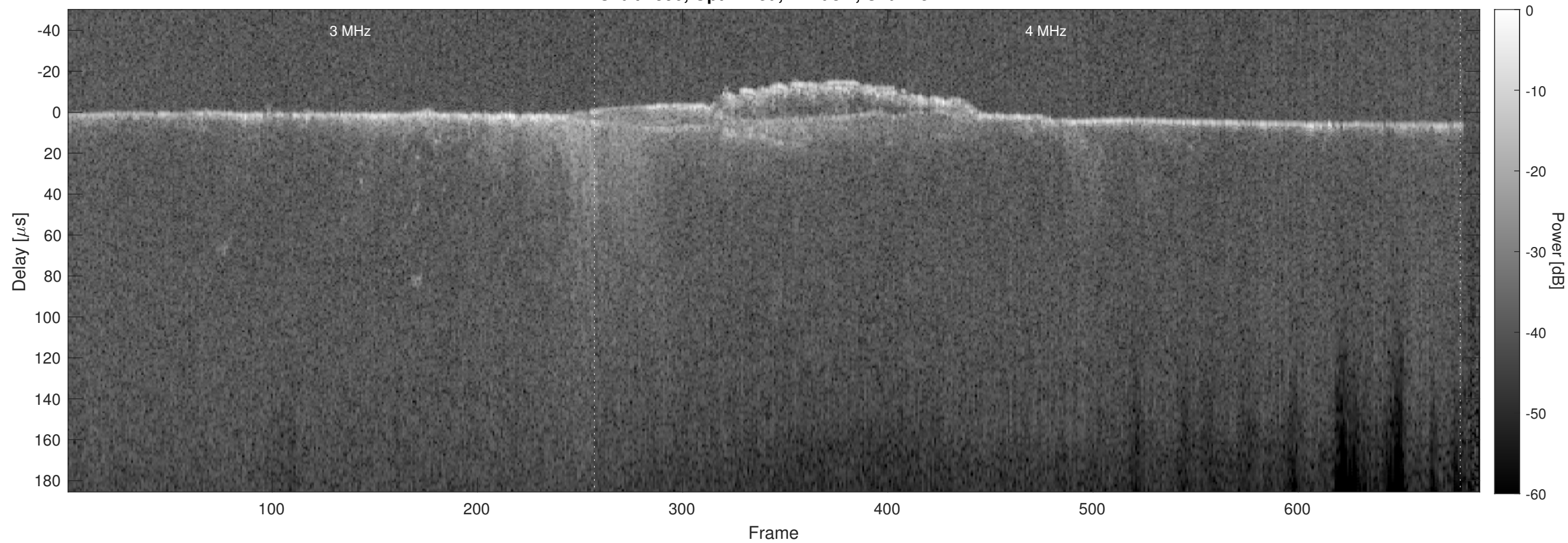
Orbit 7590, Optimized, Window, Channel 2
