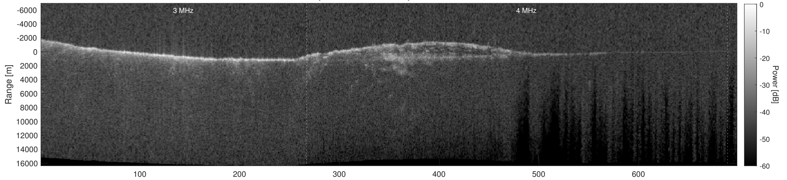
Orbit 7596, Depth-Corrected Cluttergram
