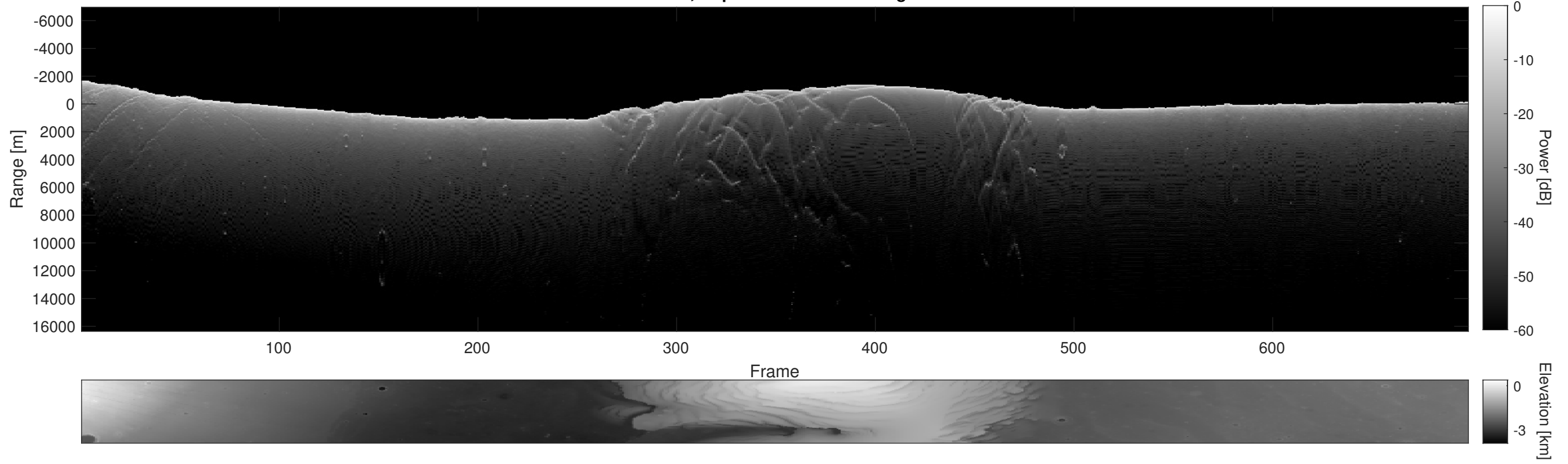
Orbit 7596, Depth-Corrected Cluttergram
