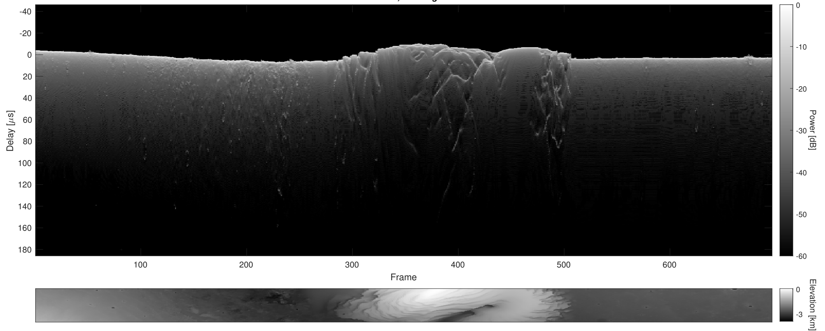
Orbit 7600, Cluttergram
