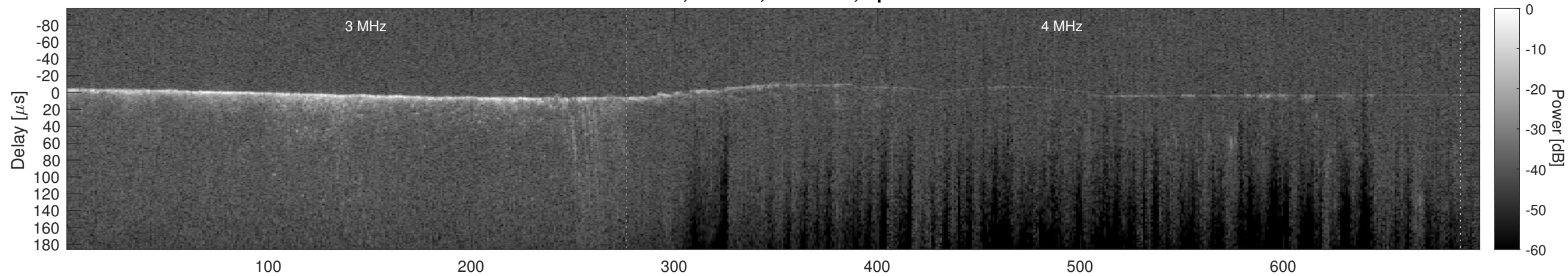
Orbit 7600, Cluttergram
