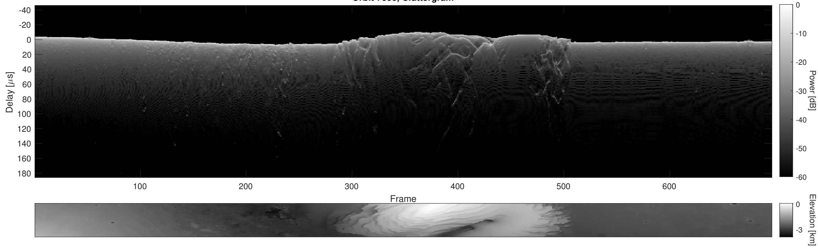
Orbit 7600, Cluttergram
