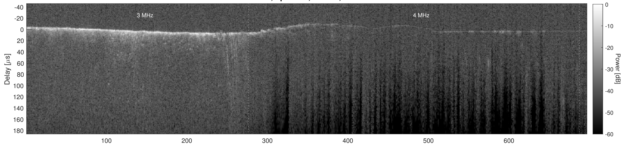
Orbit 7600, Cluttergram
