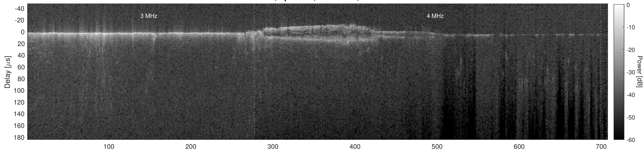
Orbit 7602, Cluttergram
