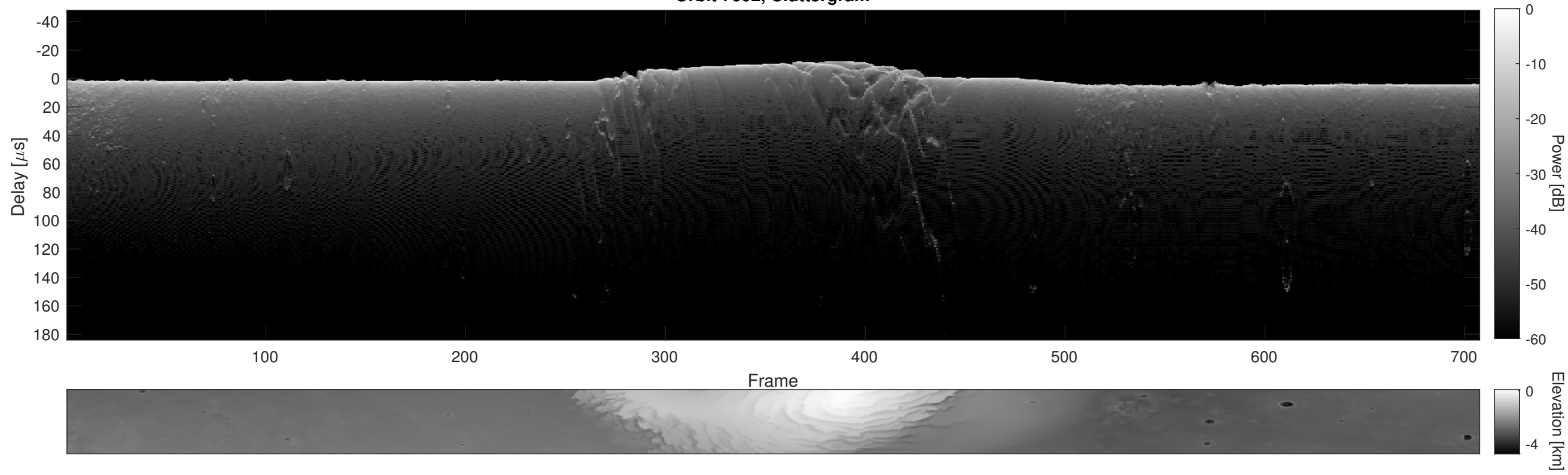
Orbit 7602, Cluttergram
