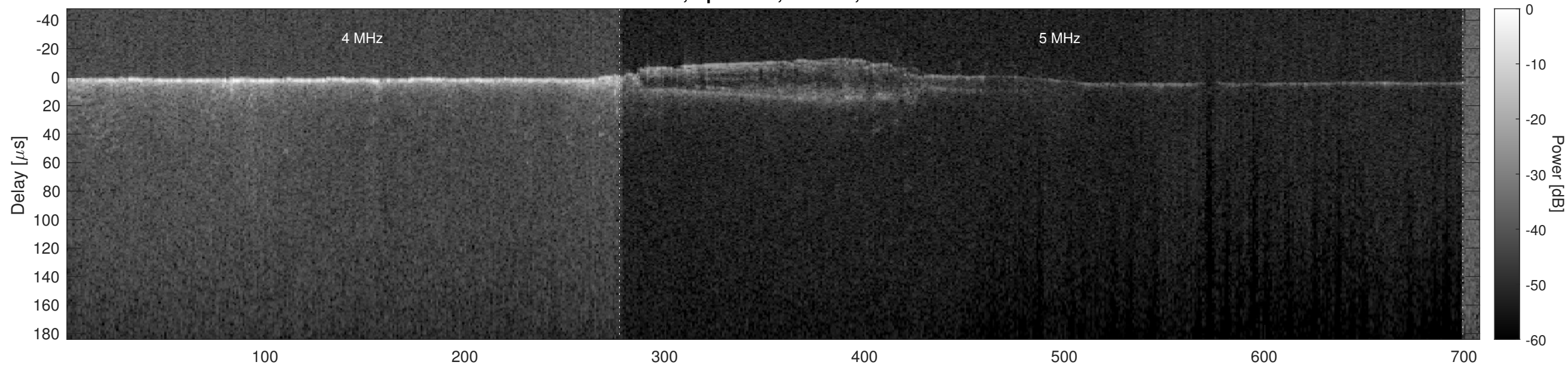
Orbit 7602, Optimized, Window, Channel 2
