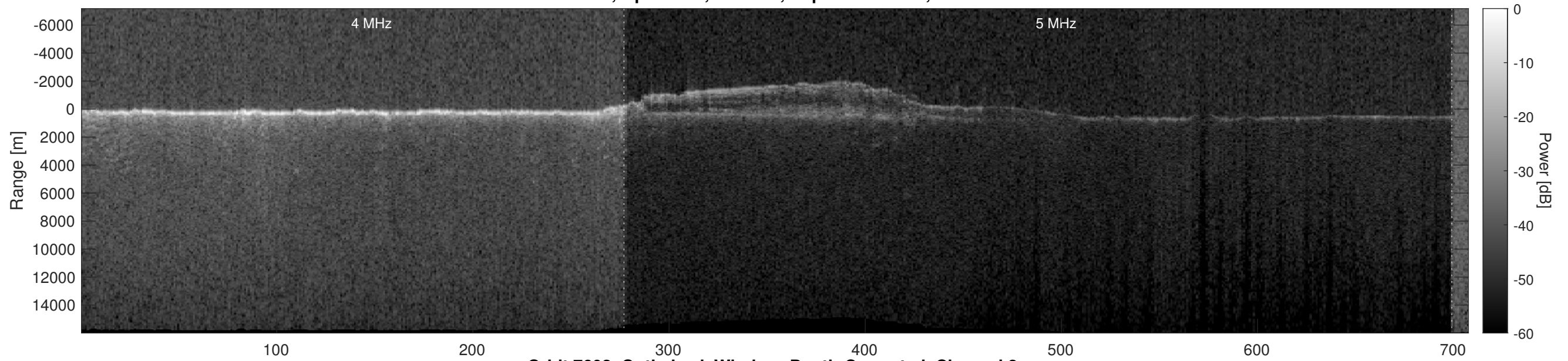
Orbit 7602, Optimized, Window, Depth-Corrected, Channel 2
