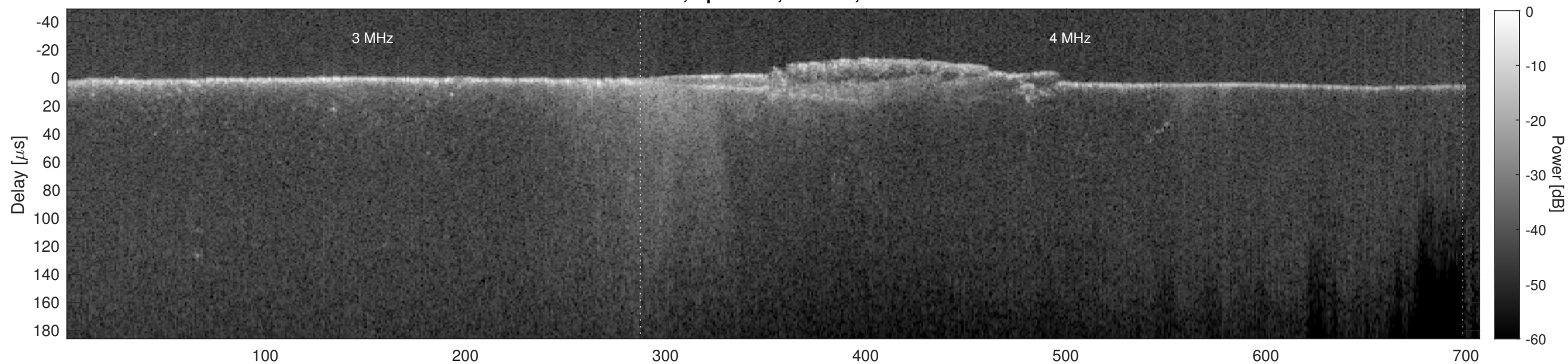
Orbit 7608, Cluttergram
