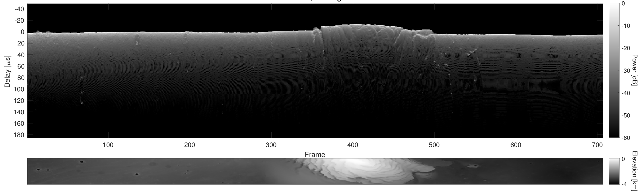
Orbit 7608, Cluttergram
