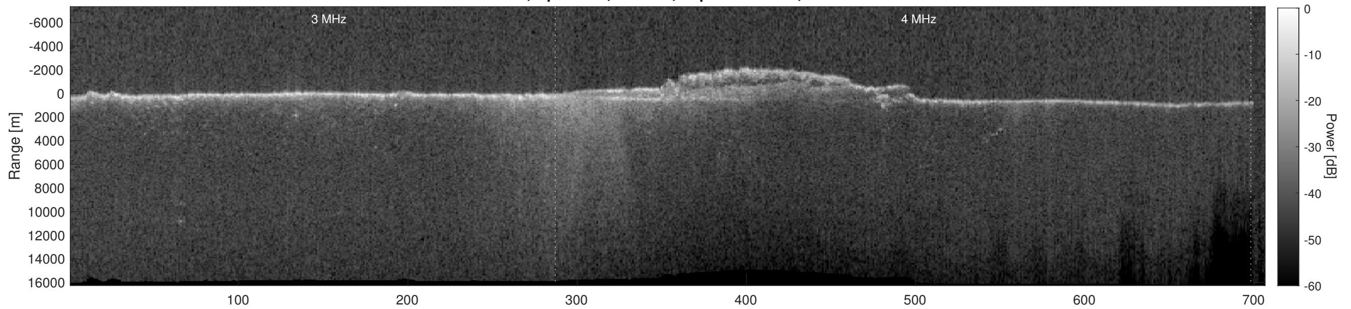
Orbit 7608, Depth-Corrected Cluttergram
