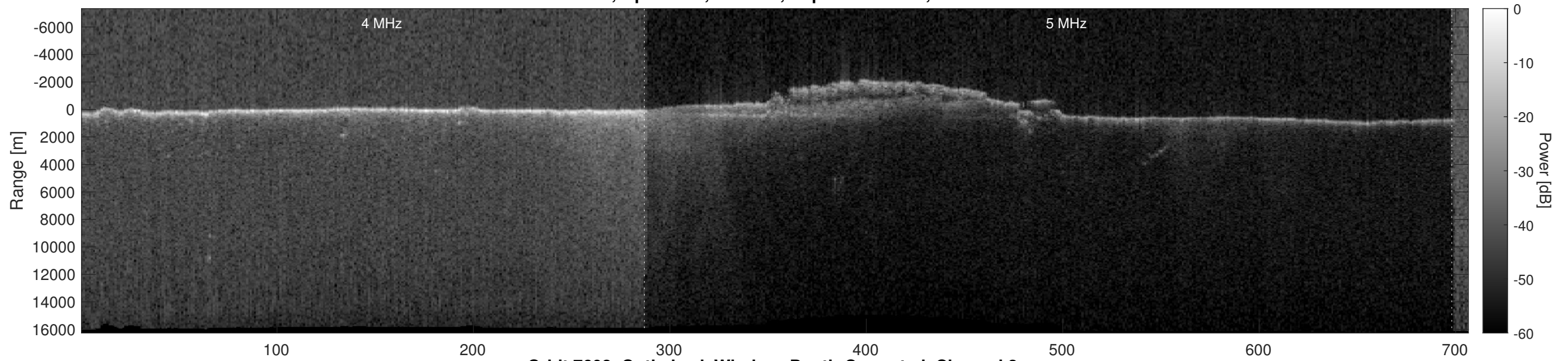
Orbit 7608, Optimized, Window, Depth-Corrected, Channel 2
