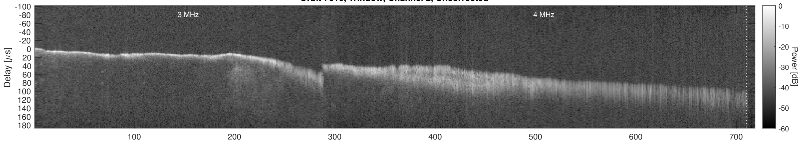
Orbit 7610, Window, Channel 2, Chapman
