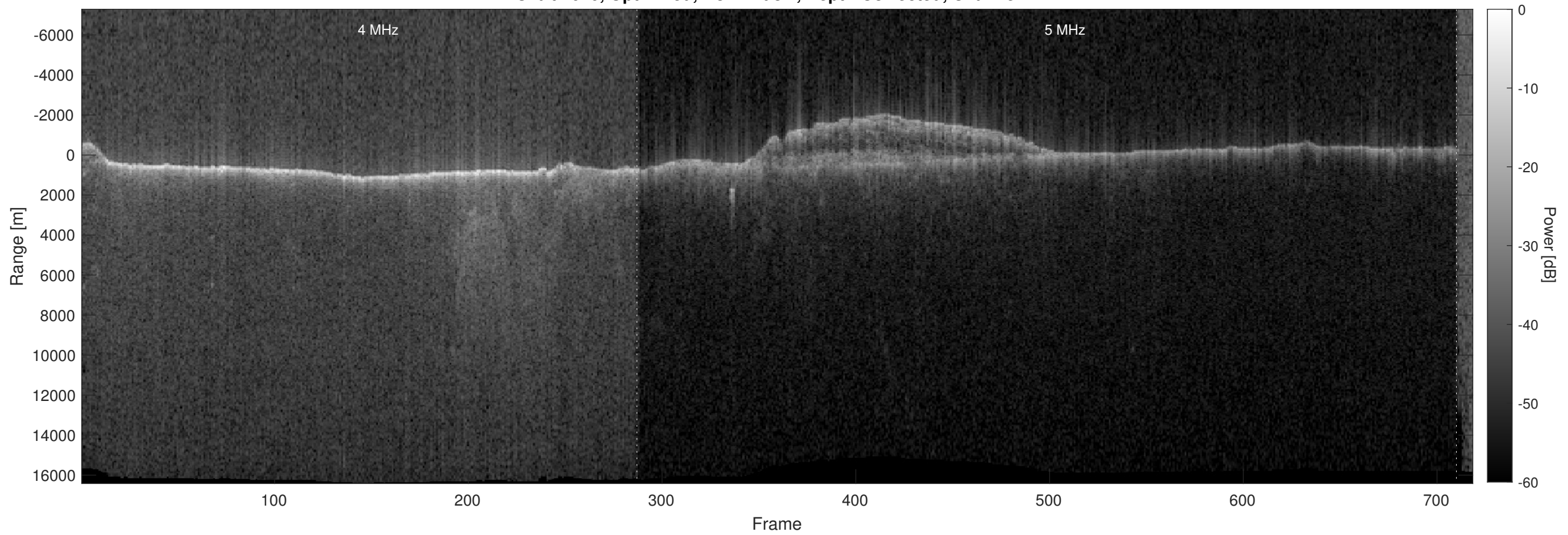
Orbit 7610, Optimized, No Window, Depth-Corrected, Channel 2
