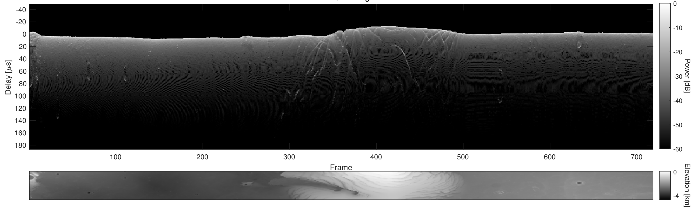
Orbit 7610, Cluttergram
