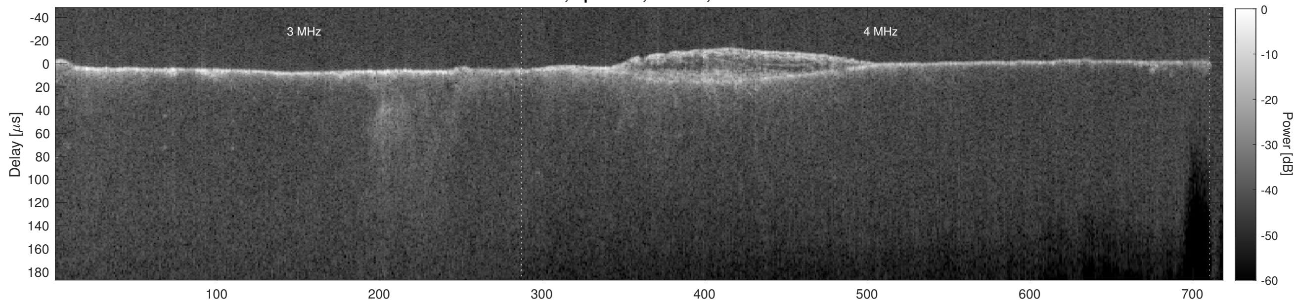
Orbit 7610, Cluttergram
