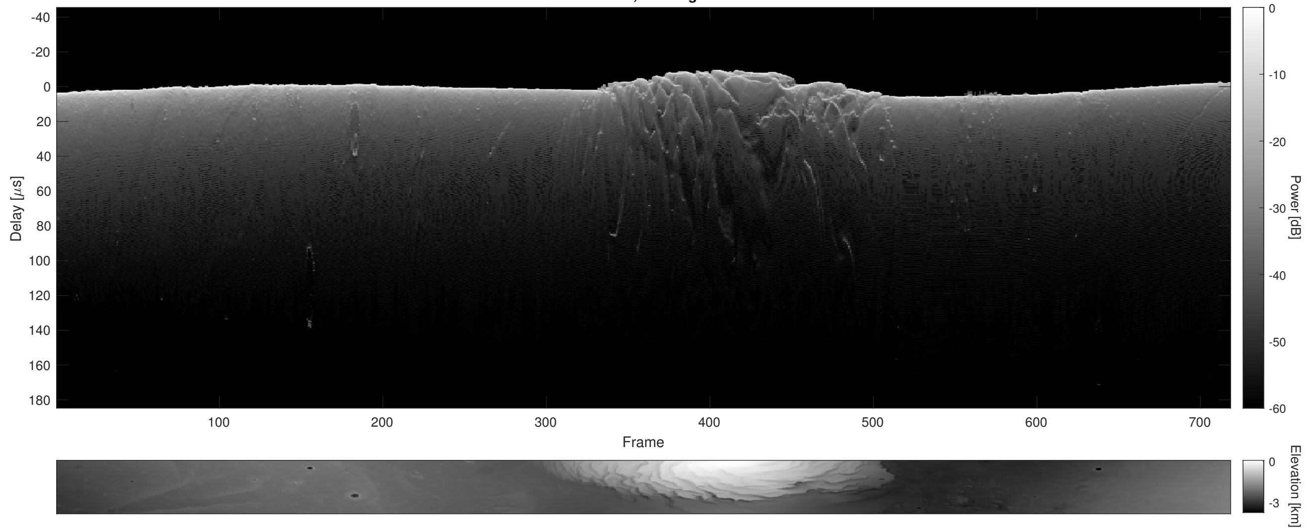
Orbit 7612, Cluttergram
