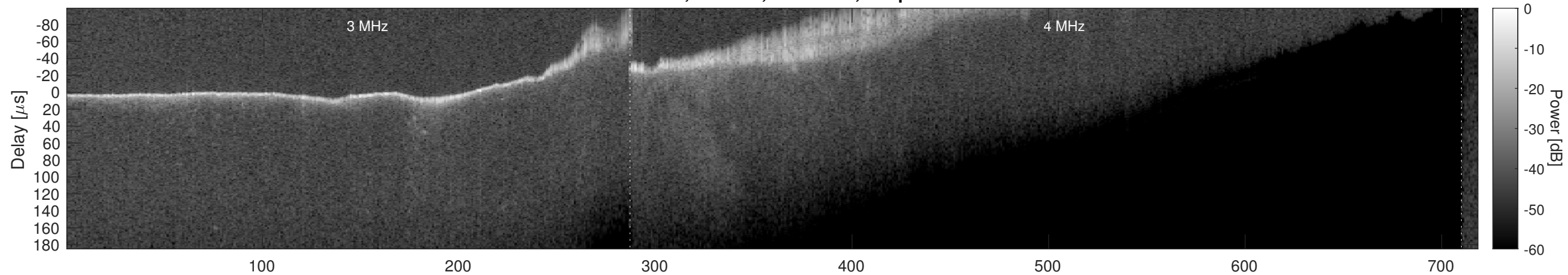
Orbit 7612, Window, Channel 2, Optimized
