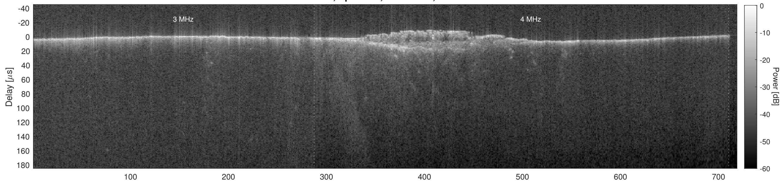
Orbit 7612, Cluttergram
