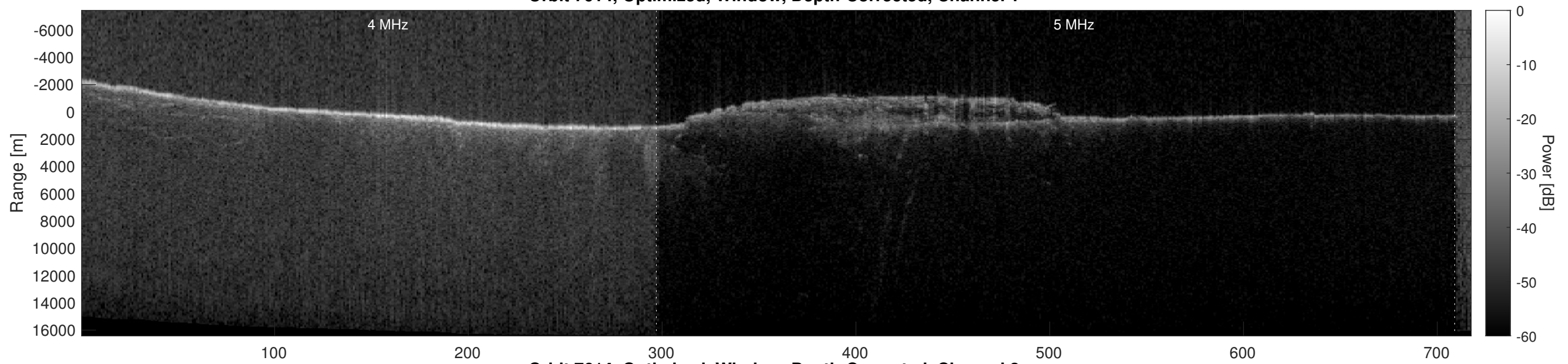
Orbit 7614, Optimized, Window, Depth-Corrected, Channel 2
