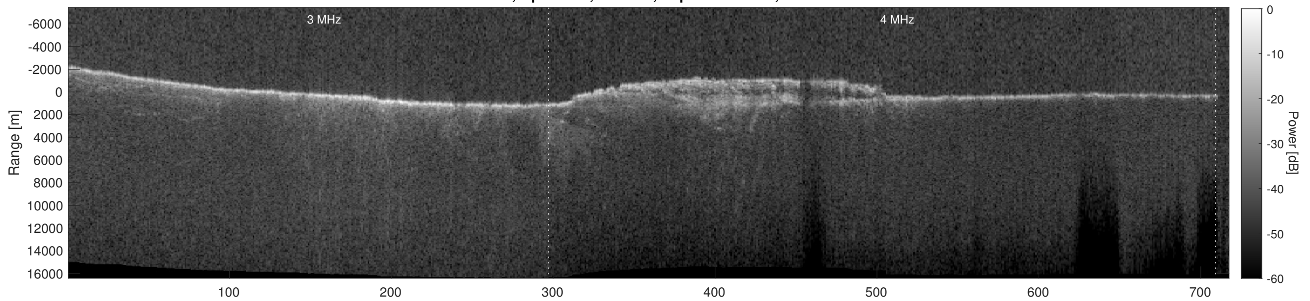
Orbit 7614, Depth-Corrected Cluttergram
