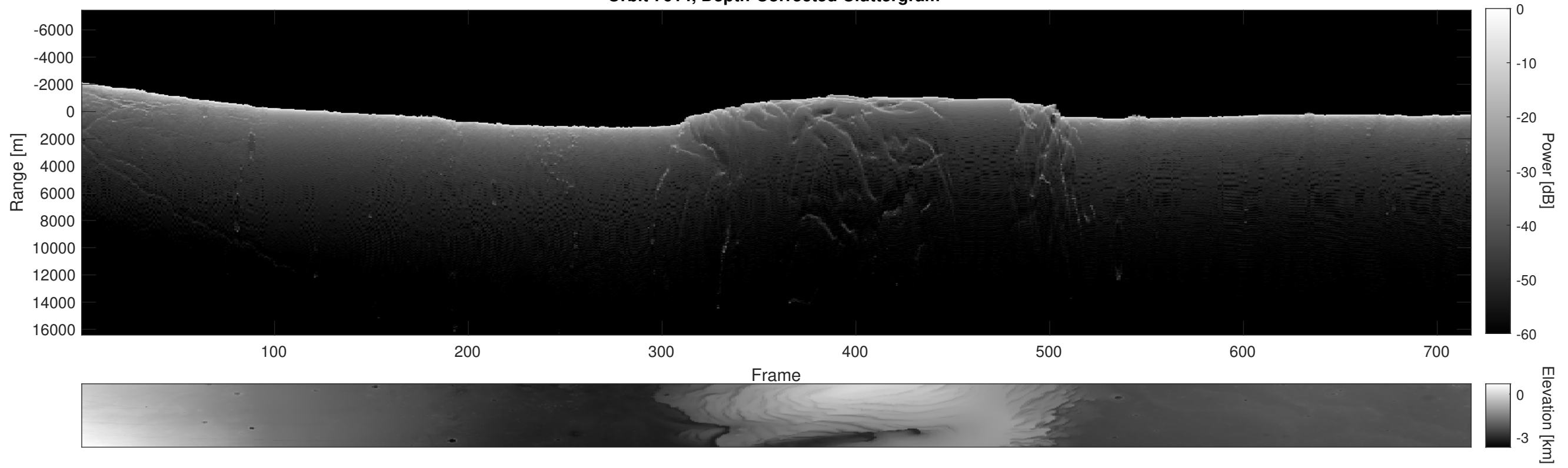
Orbit 7614, Depth-Corrected Cluttergram
