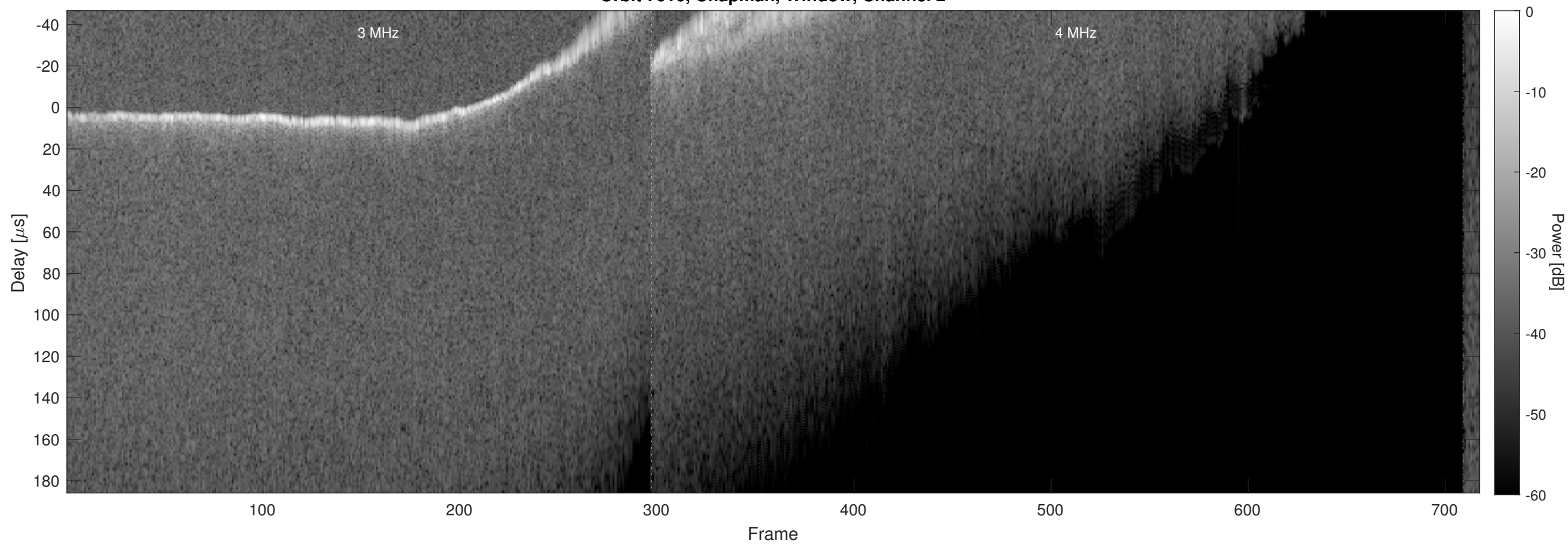
Orbit 7616, Chapman, Window, Channel 2
