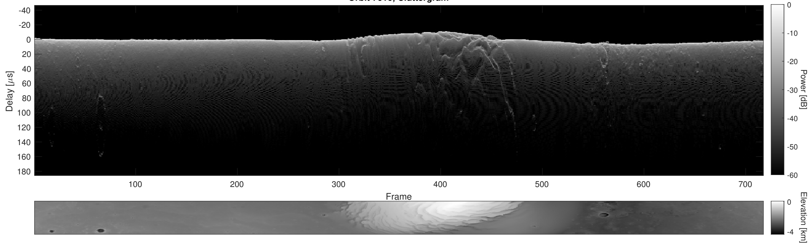
Orbit 7616, Cluttergram
