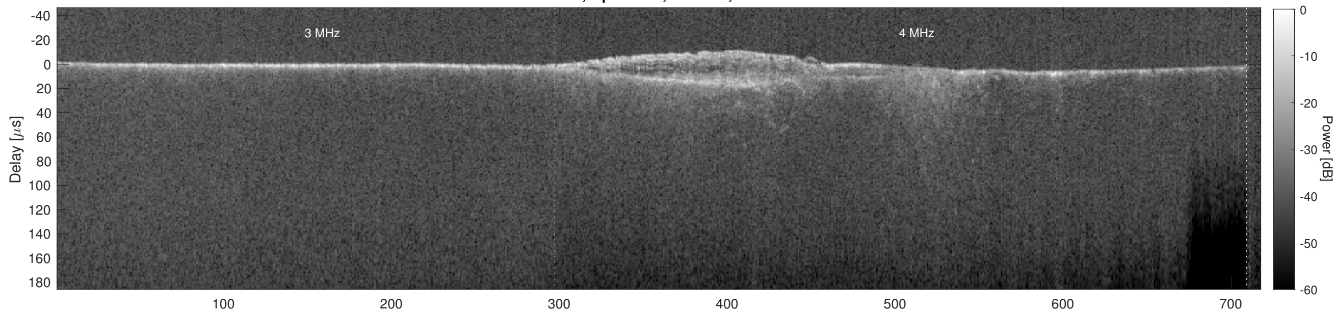
Orbit 7616, Cluttergram
