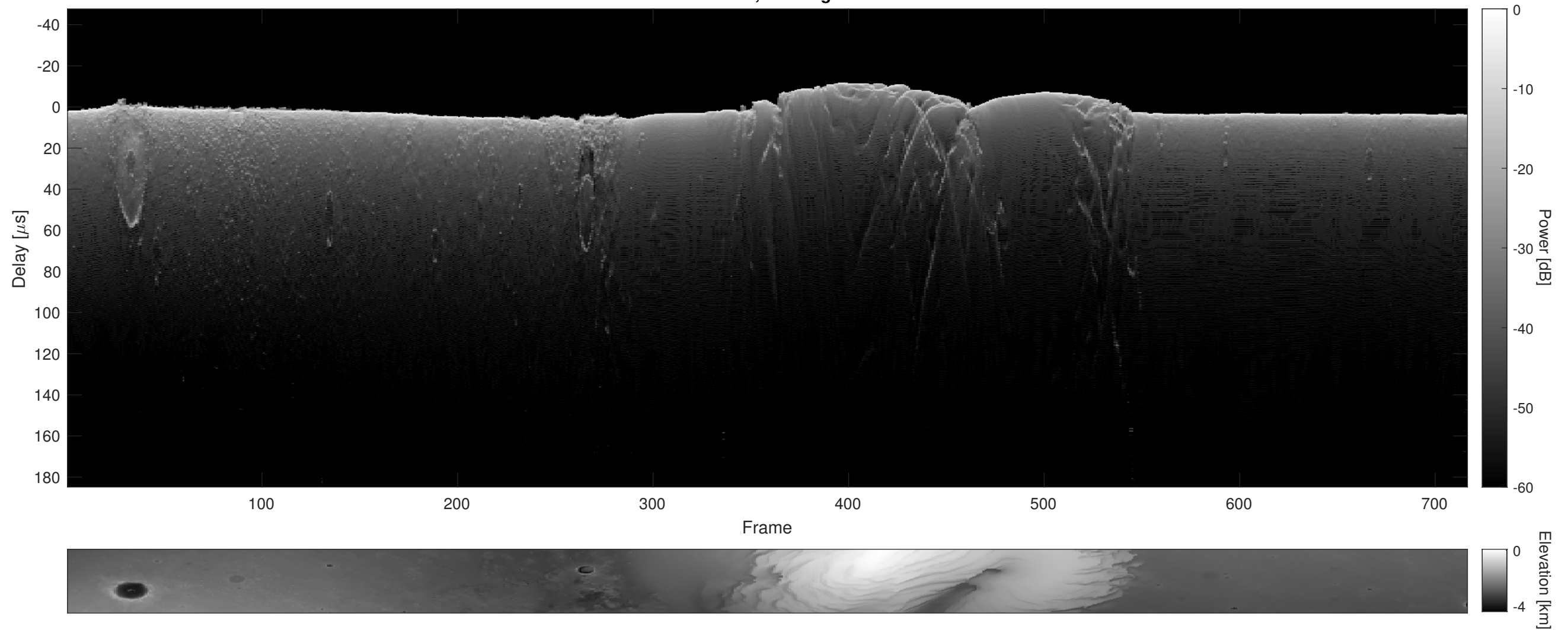
Orbit 7618, Cluttergram
