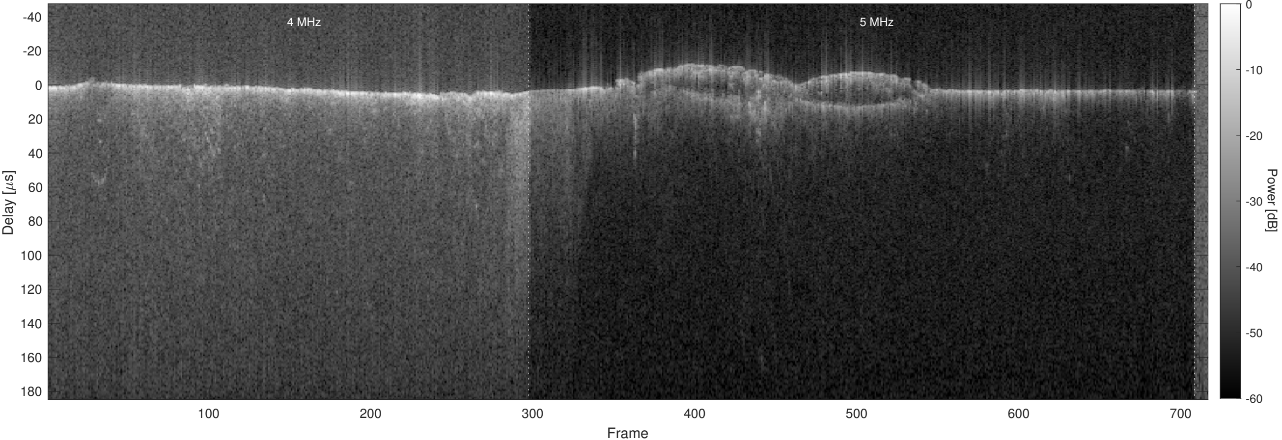
Orbit 7618, Optimized, No Window, Channel 2
