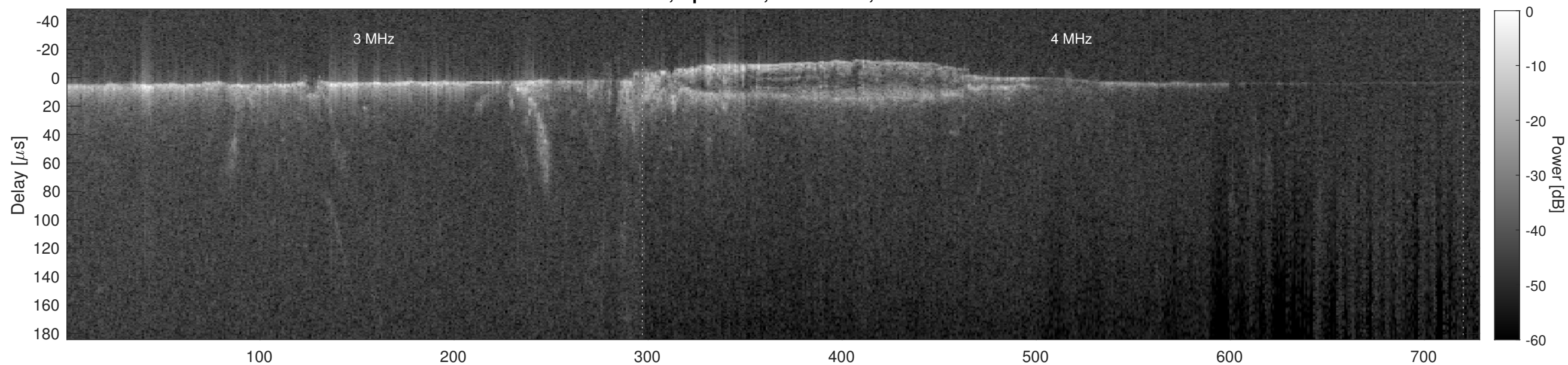
Orbit 7620, Cluttergram
