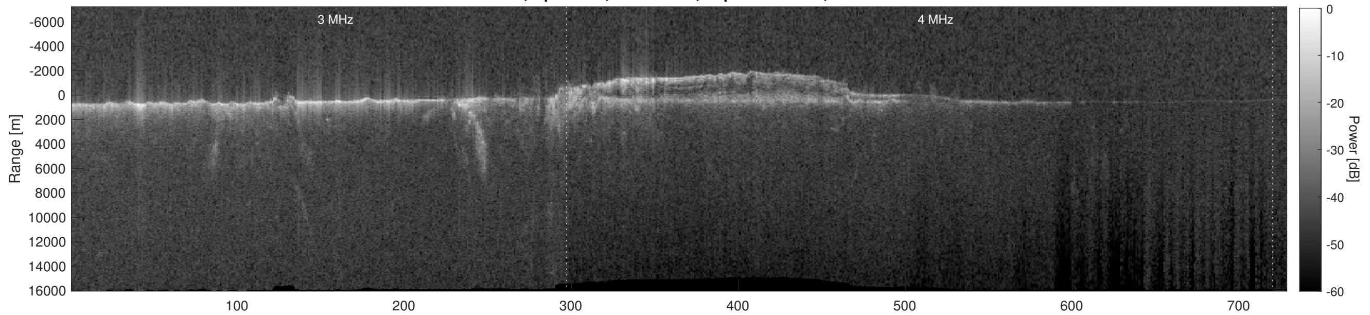
Orbit 7620, Depth-Corrected Cluttergram
