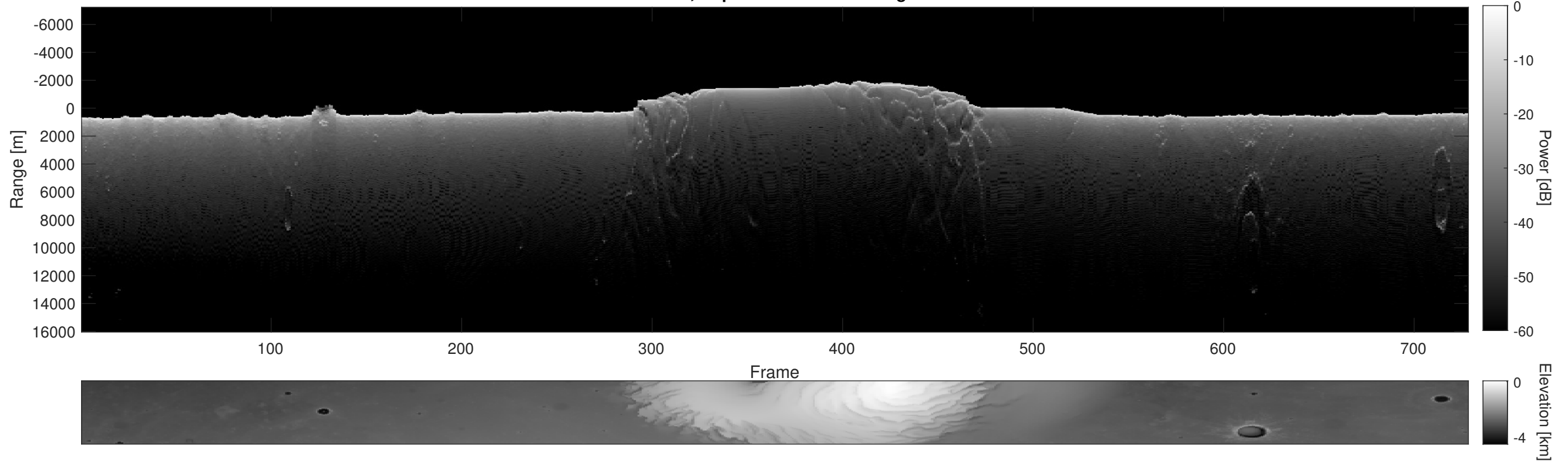
Orbit 7620, Depth-Corrected Cluttergram
