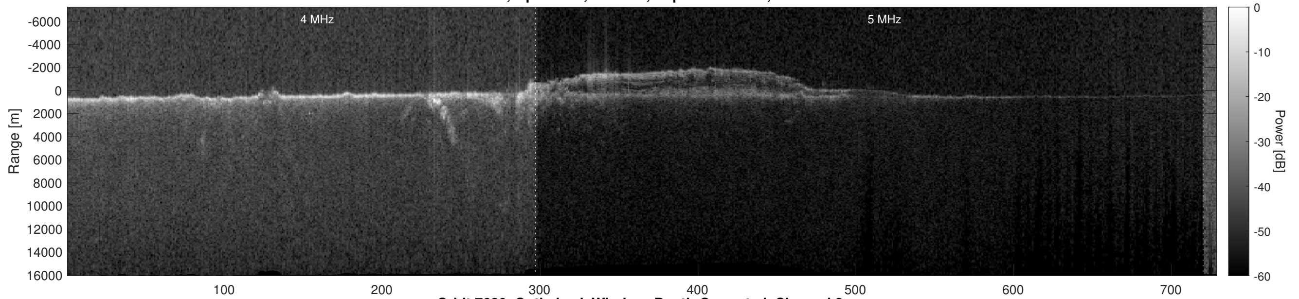
Orbit 7620, Optimized, Window, Depth-Corrected, Channel 2
