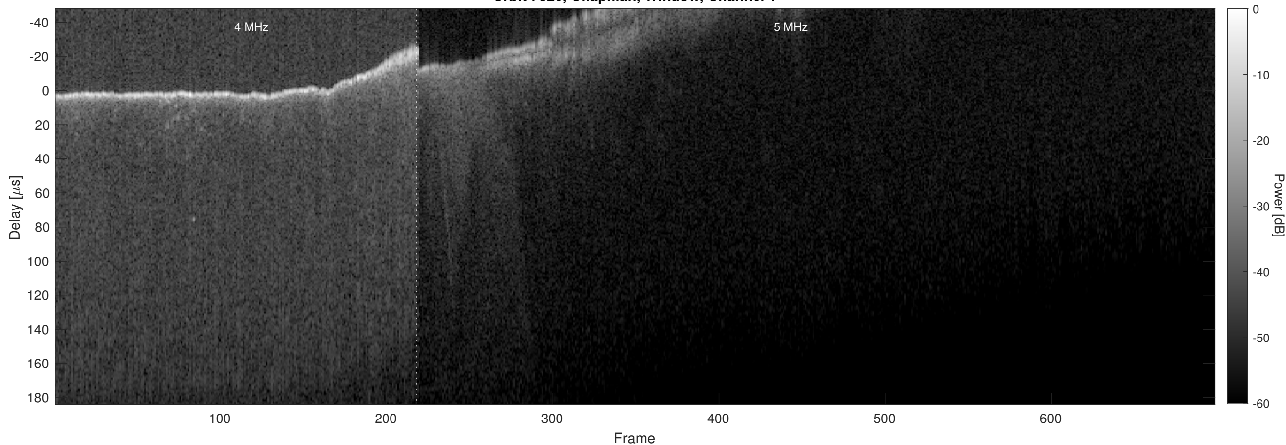
Orbit 7626, Chapman, Window, Channel 2
