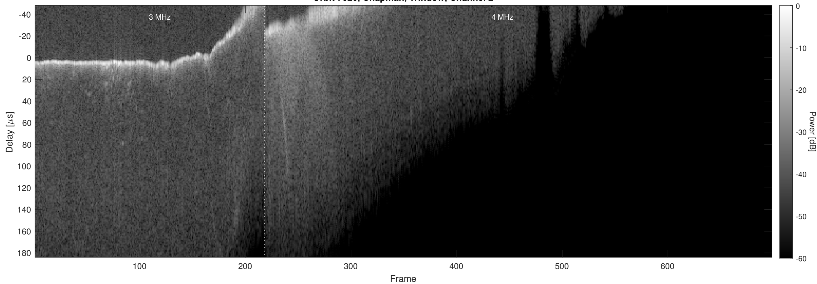
Orbit 7626, Chapman, Window, Channel 2
