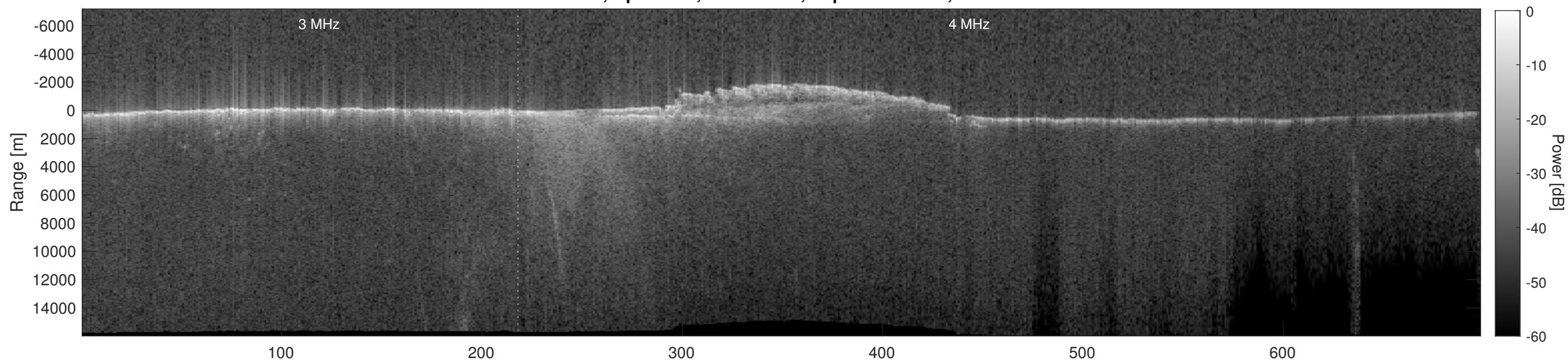
Orbit 7626, Depth-Corrected Cluttergram
