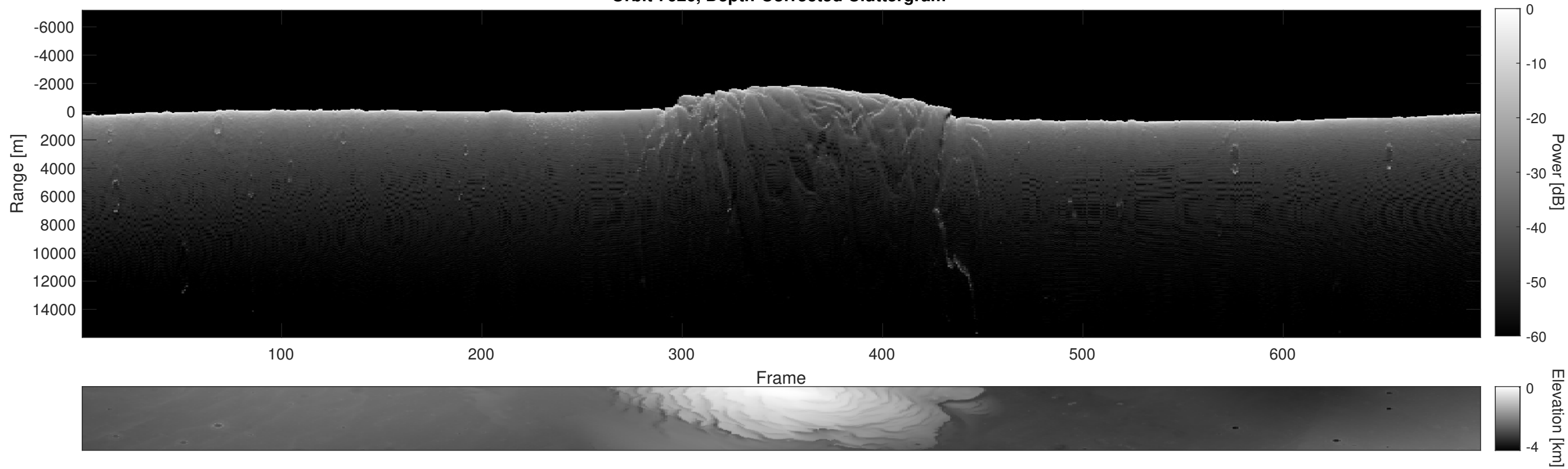
Orbit 7626, Depth-Corrected Cluttergram
